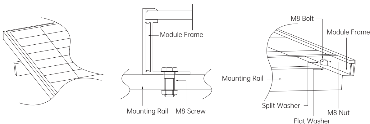
Module installed using Screw Fitting method
