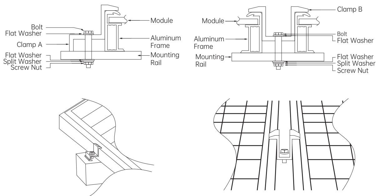
Module installed using Clamp Fitting method
