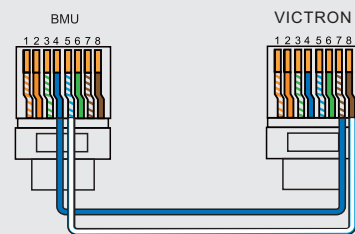
Connection with VICTRON
