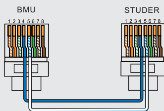
Connection with STUDER
