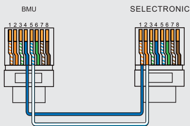
Connection with SELECTRONIC
