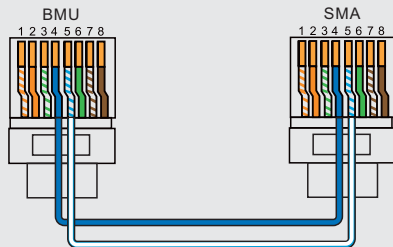
Connection with SMA
