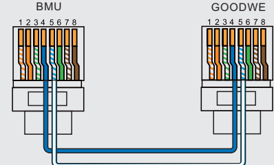
Connection with GOODWE
