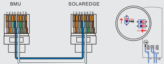
Connection with SOLAREEDGE
